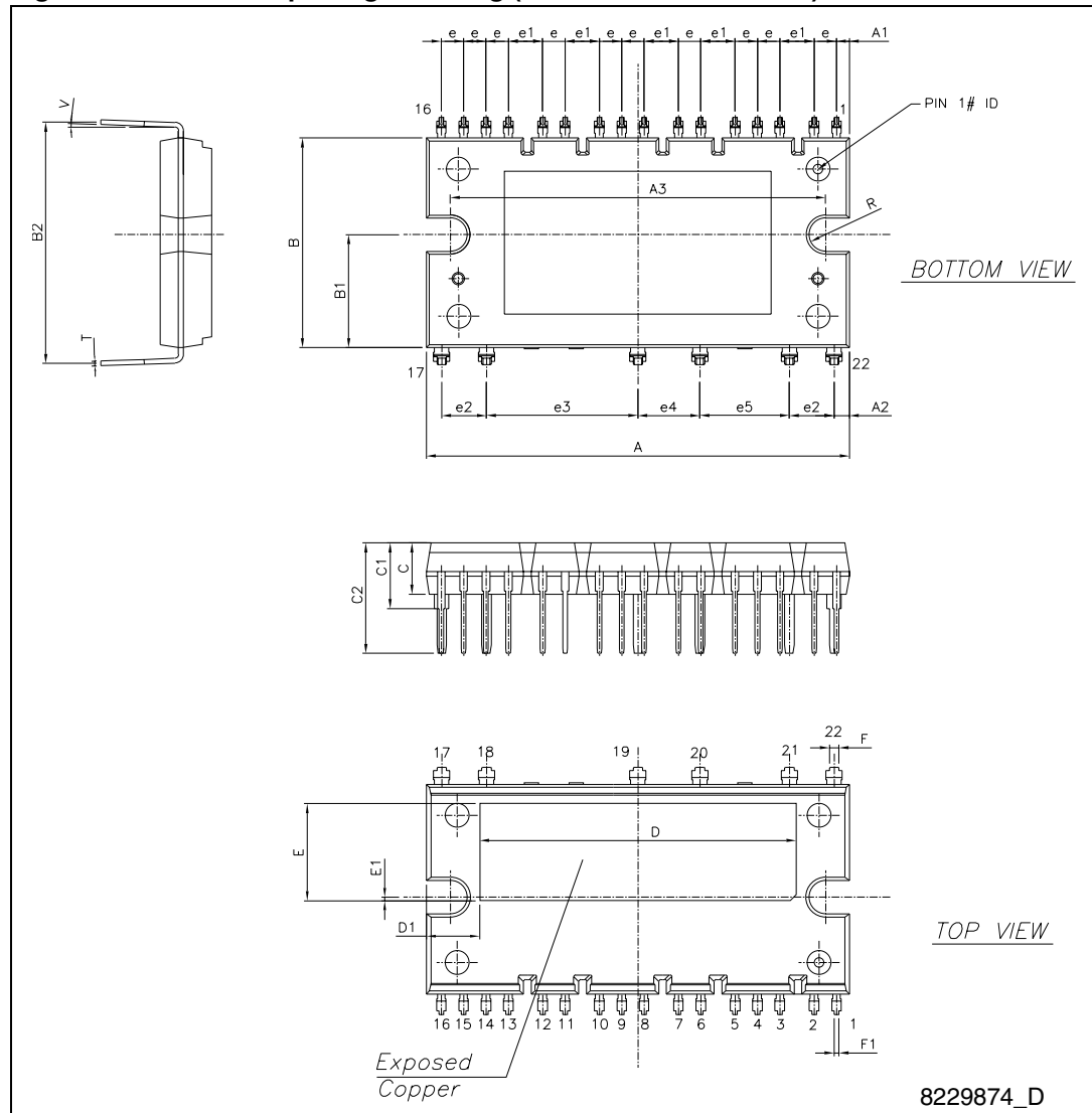
Figure 10. SDIP-22L package drawing (dimensions are in mm.)
